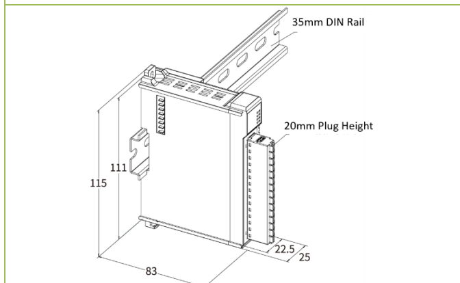
PMC-550D-X Expansion Module's 35mm DIN-Rail Installation
