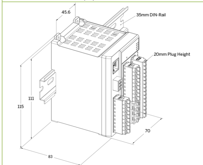
PMC-550D-X Main Unit's 35mm DIN-Rail Installation
