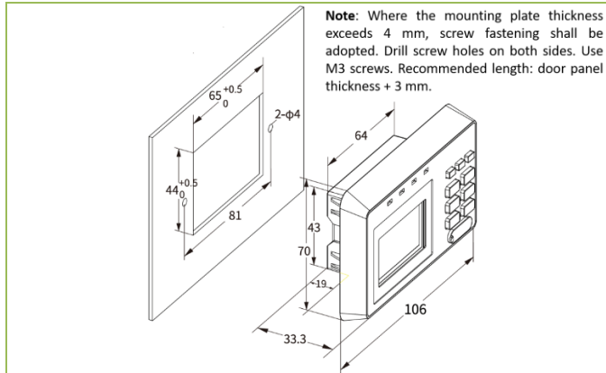
PMC-550D-X Display Module's Panel Installation
